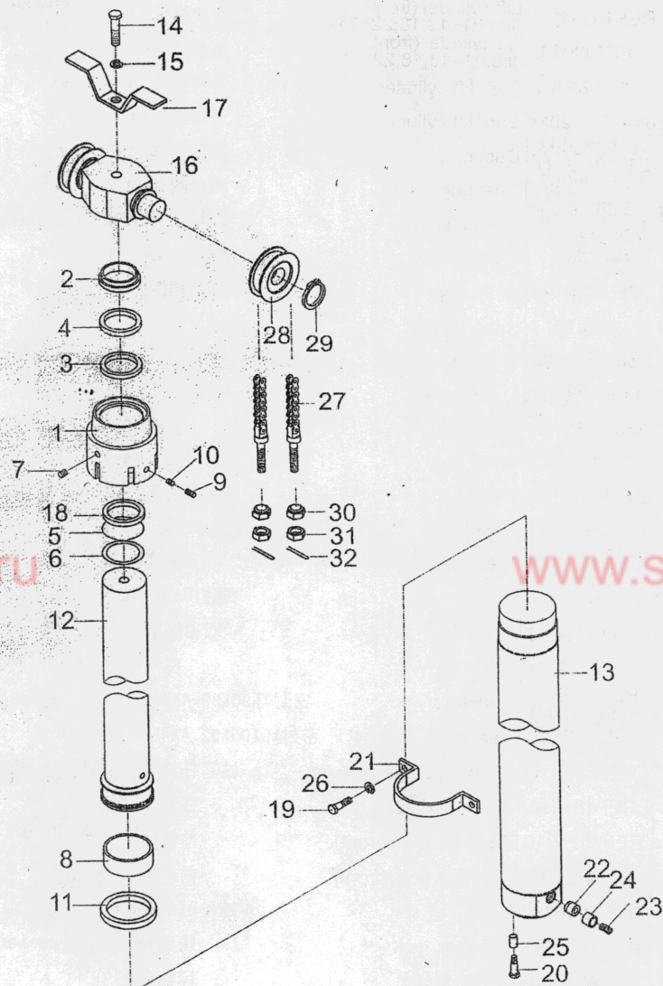
FRONT LIFT CYLINDER (FULL-FREE 2-STAGE MAST ZM)
